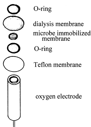
Fig. 1. Fabrication of the microbial electrode as described by Karube and Suzuki has been used [26].
