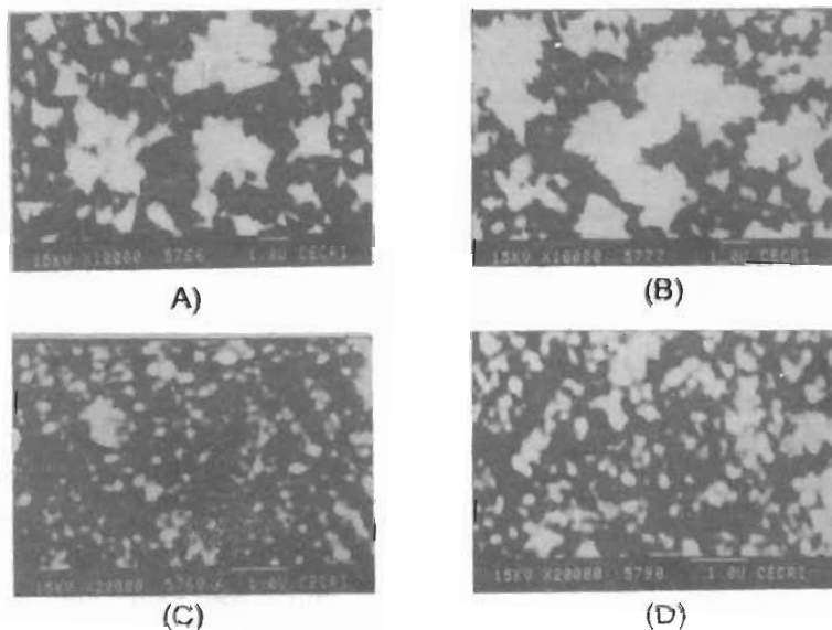
Fig. 1: SEM micrographs taken on Ni-Co black coatings deposited using (a) 3.53 A.dm -2 for 50 sec (b) 4.7 A.dm -2 for 50 sec (c) 5.9 A.dm -2 for 20 sec (d) for 30 sec
