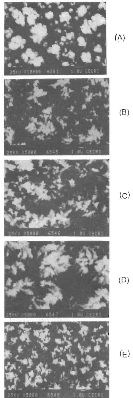
Fig. 2: SEM micrographs taken on Ni-Co black coatings deposited using (a) 3.53 A.dm -2 for 30 sec (b) 8.2 A.dm -2 for 20 sec (c) 8.2 A.dm -2 for 40 sec (d) 8.2 A.dm -2 for 50 sec and (e) 9.4 A.dm -2 for 20 sec with sputtered film of gold on the surface
