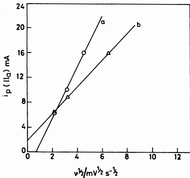
Fig. 6: Linear dependence of i_p of peak II_a on \nu^{1/2} for alloy I to III in 0.5 M NaCl a) alloy I b) alloy II
