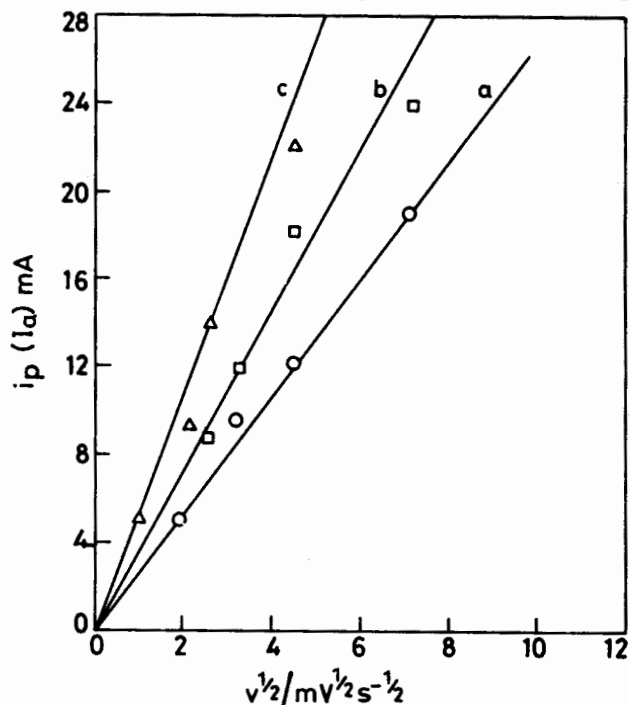
Fig.5: Linear dependence of i_p of peak I a on v^{1/2} for alloy I to III in 0.5 M NaCl a) alloy I b) alloy II c) alloy III
