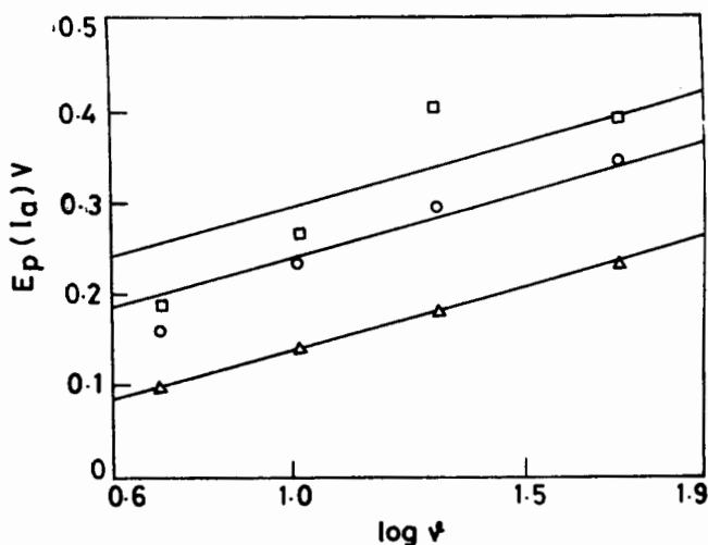
Fig.7: Relationship between E_p and \log \nu for given alloys I to III in 0.5 M NaCl a) alloy I b) alloy II c) alloy III
