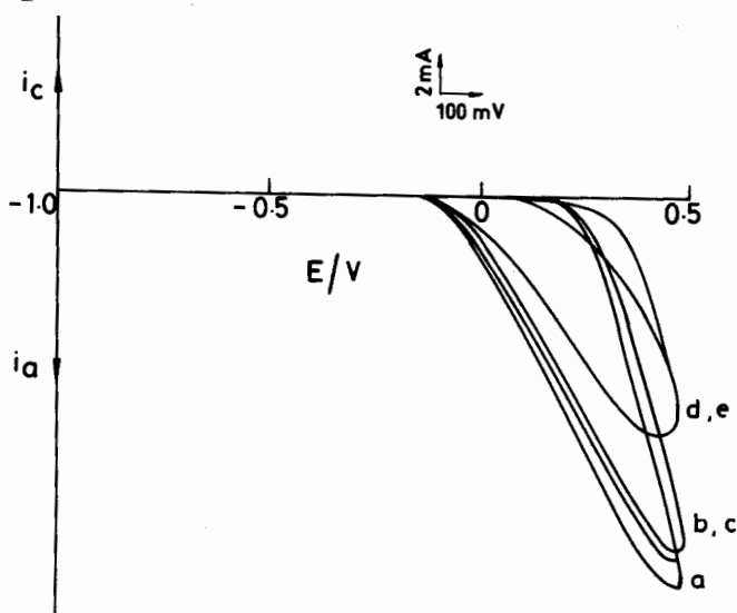
Fig. 1: Cyclic voltammogram of pure nickel in 0.5 M NaCl at different sweep rates a) 5 mV/s b) 10 mV/s c) 20 mV/s d) 50 mV/s e) 100 mV/s
