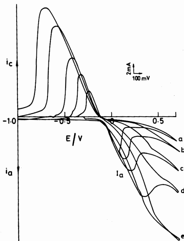
Fig. 2: Cyclic voltammogram of pure copper in 0.5 M NaCl at different sweep rates a) 5 mV/s b) 10 mV/s c) 20 mV/s d) 50 mV/s e) 100 mV/s
