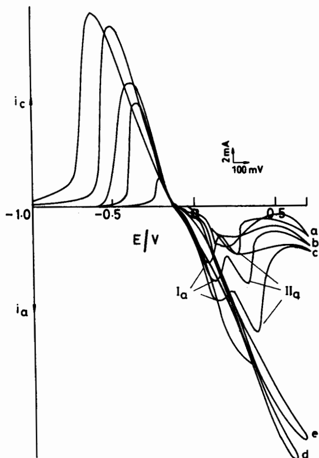
Fig.4: Cyclic voltammogram of alloy I in 0.5 M NaCl at different sweep rates a) 5 mV/s b) 10 mV/s c) 20 mV/s d) 50 mV/s e) 100 mV/s
