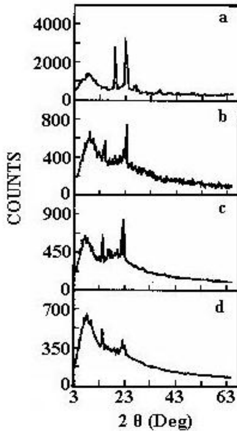
Figure 1. XRD patterns for: a) Pure PEO, b) (\text{PEO})_8\text{-LiAsF}_6 , c) (\text{PEO})_8\text{-LiAsF}_6\text{-(DBS)}_{0.4} ; d) (\text{PEO})_8\text{-LiAsF}_6\text{-(DBS)}_{0.4}\text{-(EC)}_{0.1} .
