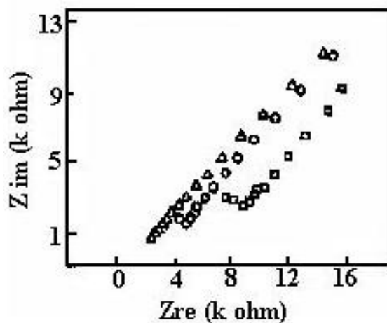
Figure 8. Impedance diagram for (PEO) 8 -LiAsF 6 -(DBS) 0.4 -(EC) 0.1 at 45 °C (□), at 55 °C and at 65 °C (Δ).
