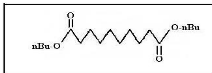
Structure of Dibutyl Sebacate
