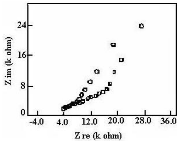
Figure 7. Impedance diagram for (PEO) 8 -LiAsF 6 at 55 °C (□) and at 65 °C (○).
