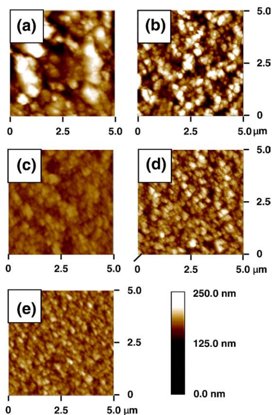
Fig. 1. AFM images of PEDOT films with various Im/EDOT molar ratios: (a) 0, (b) 1.0, (c) 1.5, (d) 2.0 and (e) 2.5.
