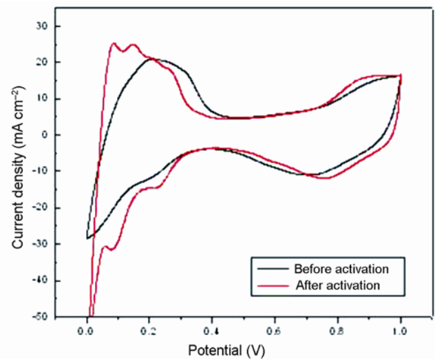
Figure 4. CVs for Pt/PEDOT-PSSA recorded at 25^\circ\text{C} in a single cell with \text{H}_2 and \text{N}_2 streams at anode and cathode, respectively (scan rate = 50 \text{ mV s}^{-1} ) before and after the galvanostatic polarization of PEFC at 60^\circ\text{C} .
